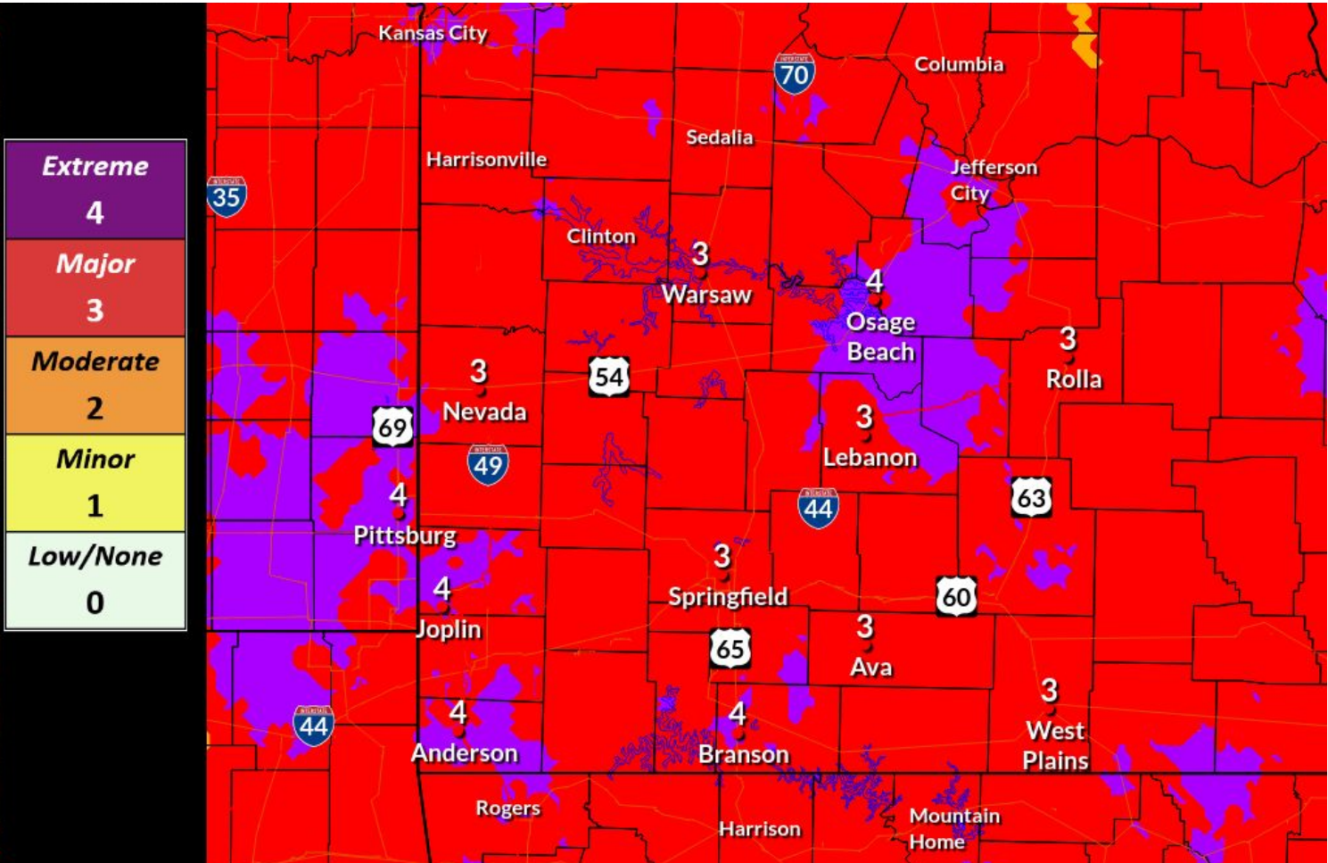
HeatRisk Wednesday
