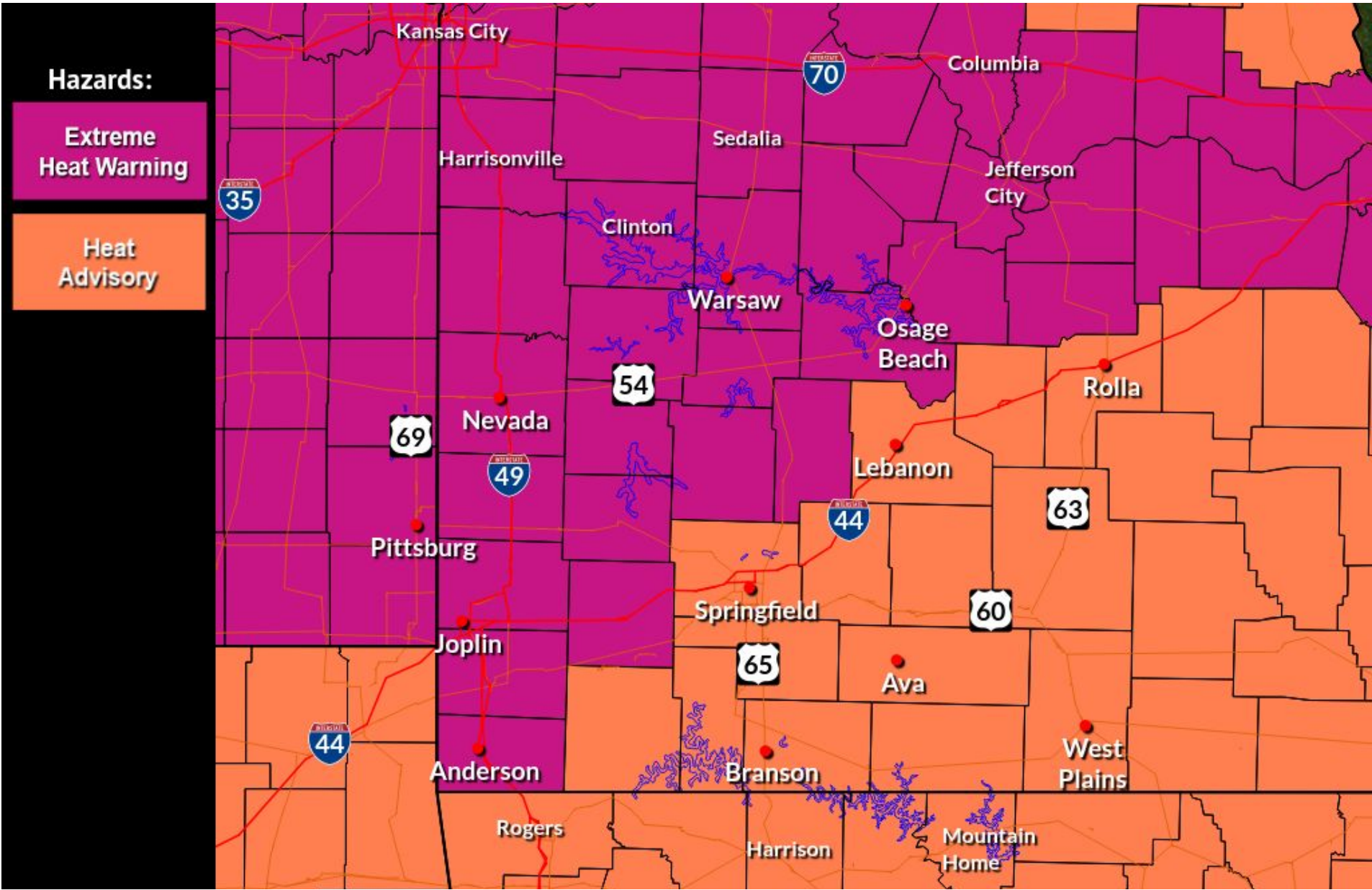
Heat Headlines
