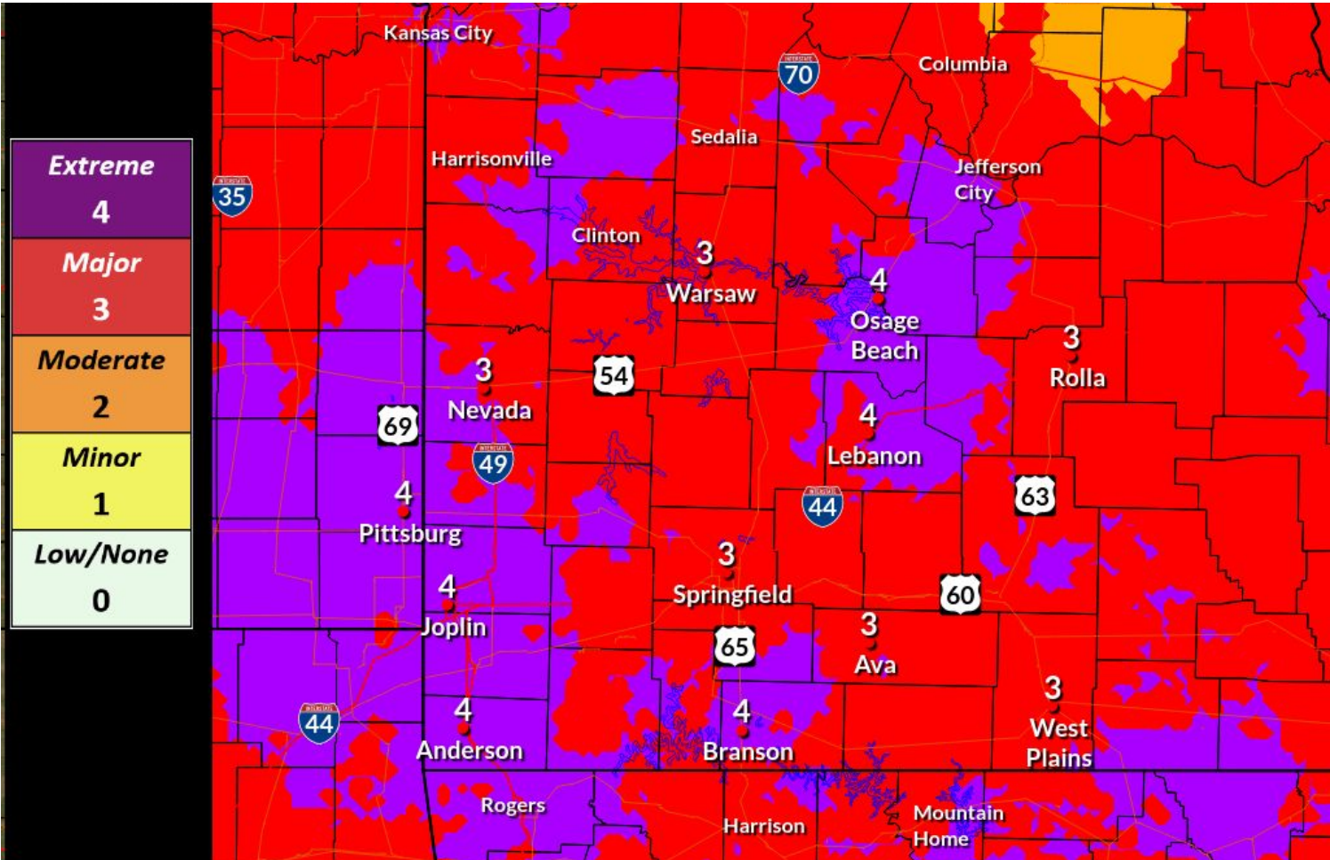
HeatRisk Thursday
