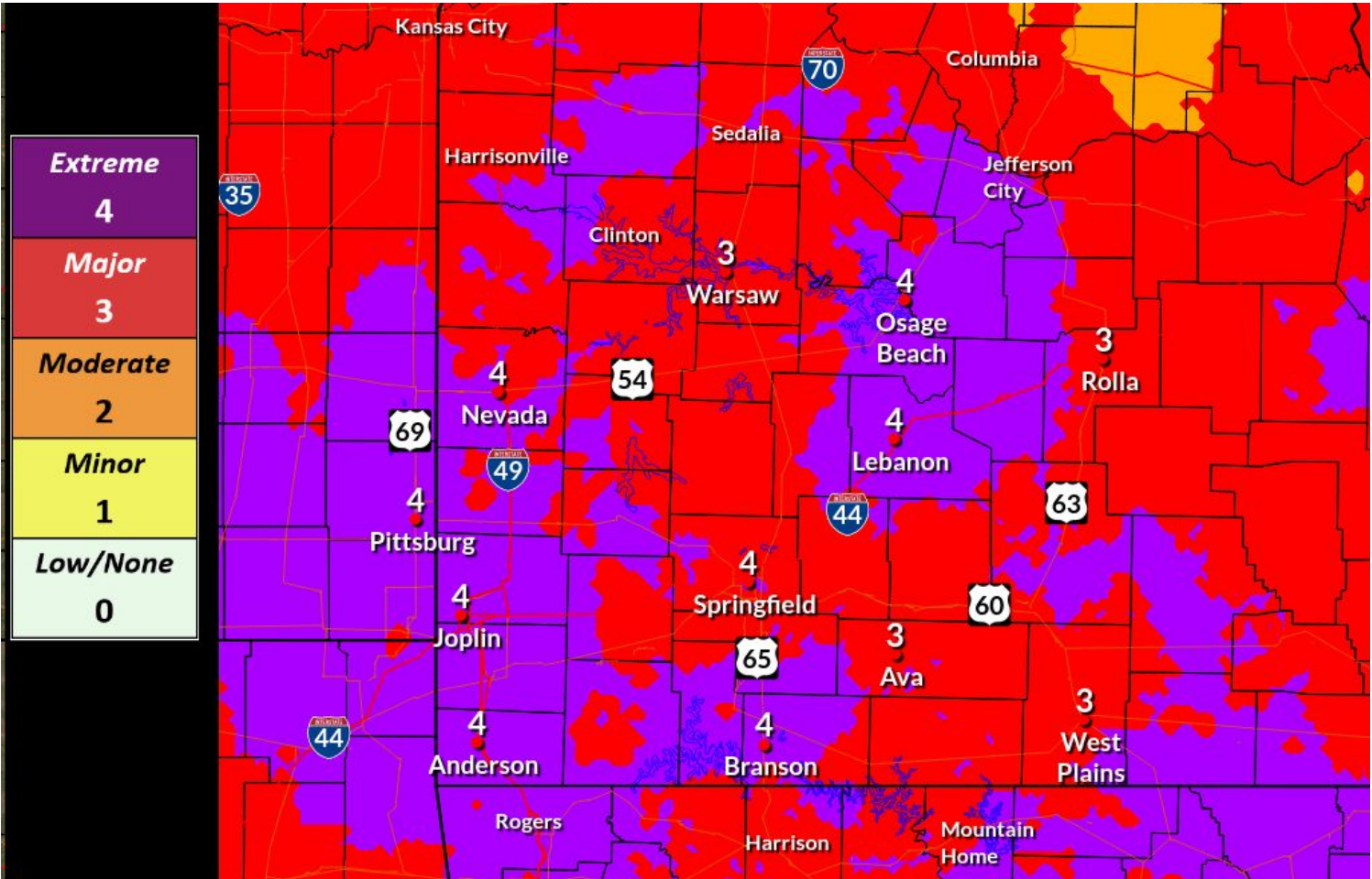
HeatRisk Friday
